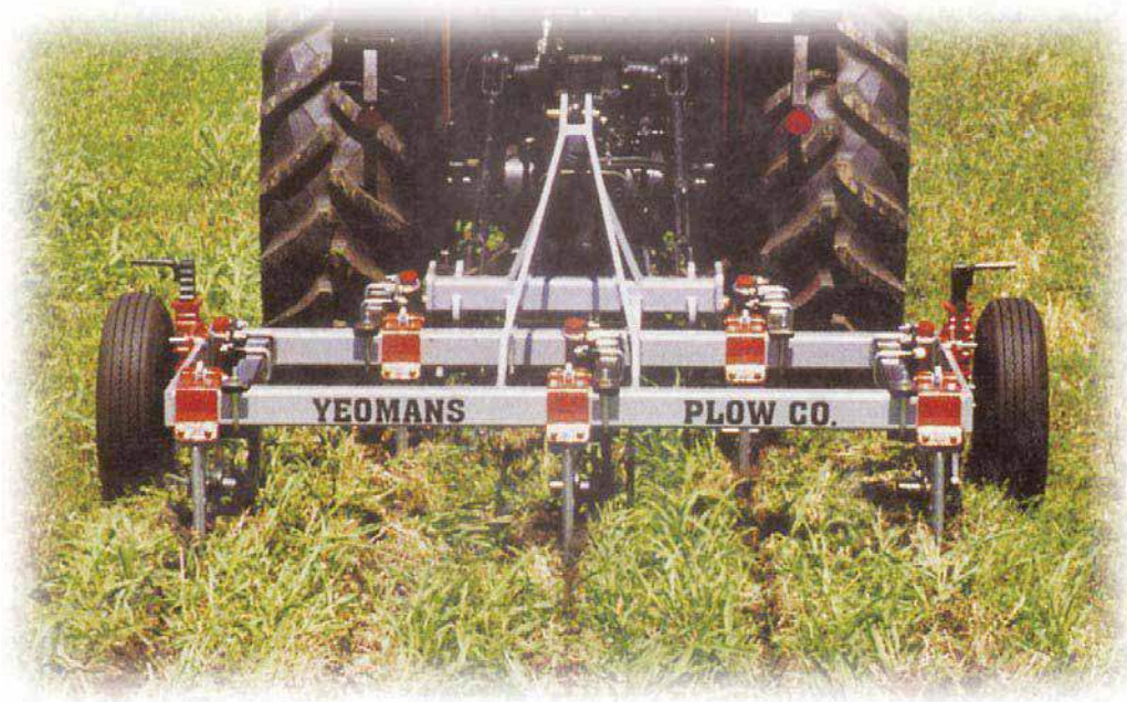
GP39-8 Frame - In Action. The GP39-8 set up with Depth Wheels, five 22" Shanks and 16" Coulters
